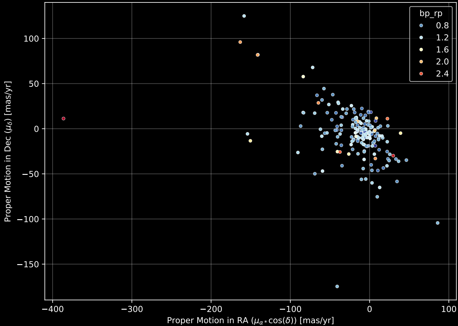
APOGEE DR17 Field: [029+77_MGA] Proper Motion Diagram (n= 184)
