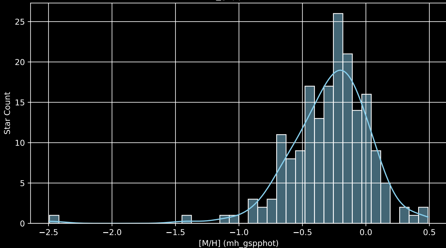
APOGEE DR17 Field: [029+77_MGA [M/H] (mh_gspphot) (n= 183)
