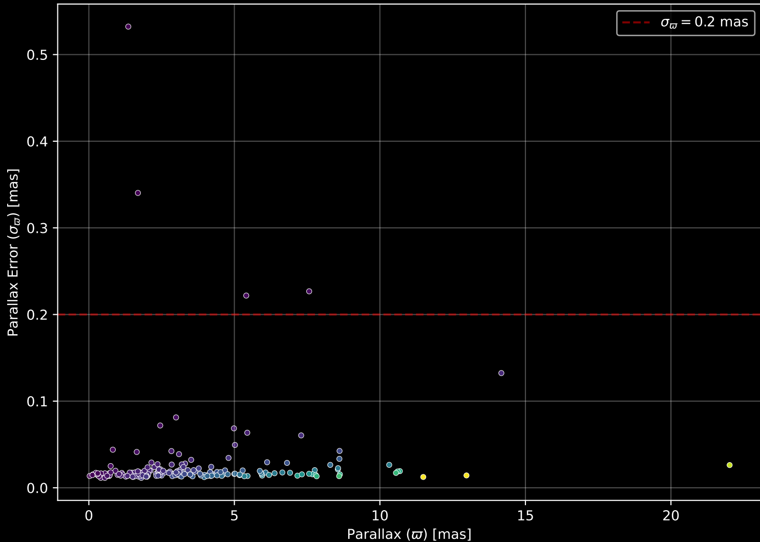
APOGEE DR17 Field: [029+77_MGA] Parallax Quality (n= 184)
