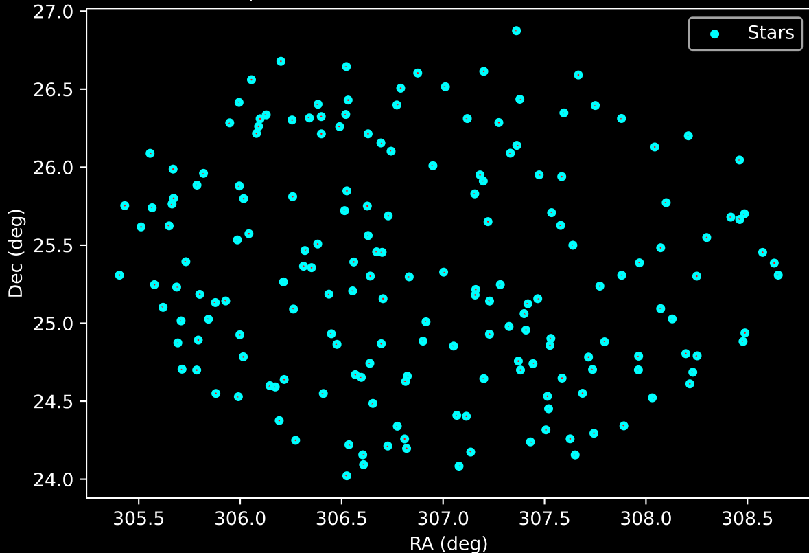
APOGEE DR17 Field: [029+77_MGA] Proper Motion Vectors for Gaia Star Field (n= 184)
