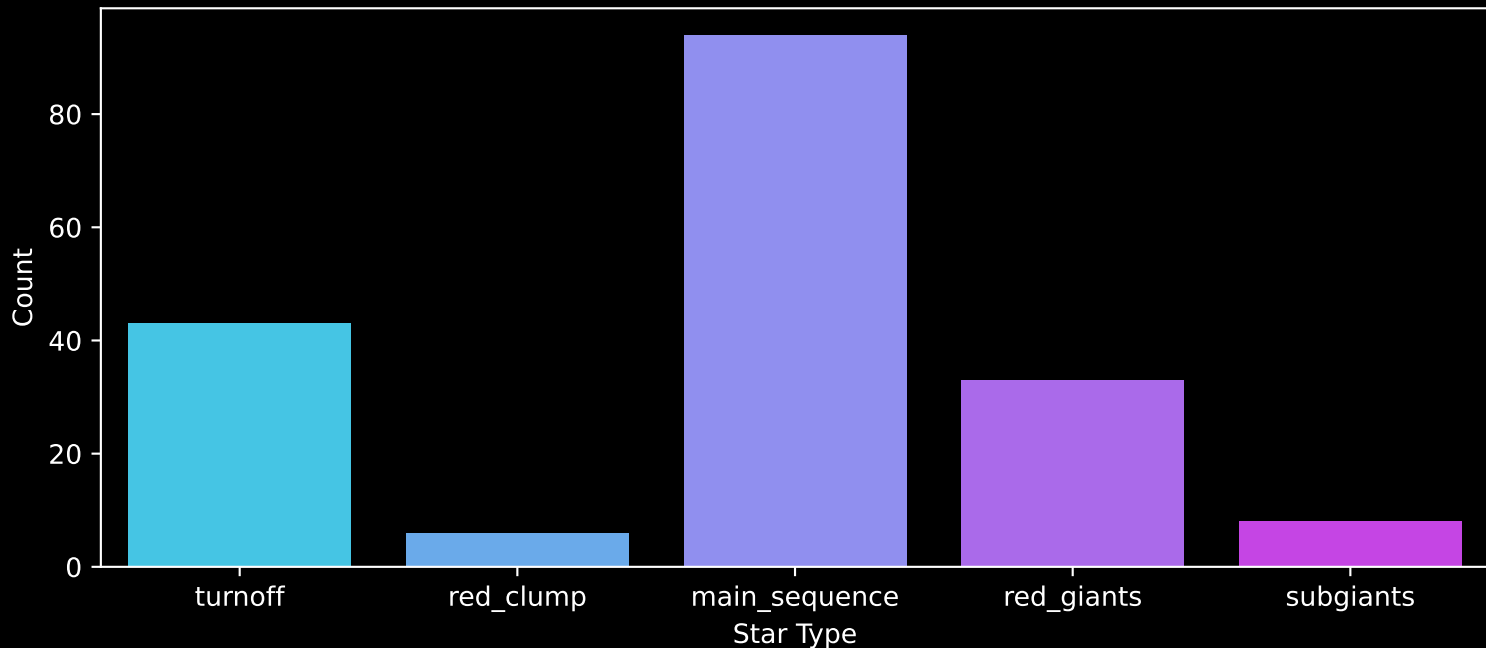
APOGEE DR17 Field: [029+77_MGA] Count plot of Star Type
