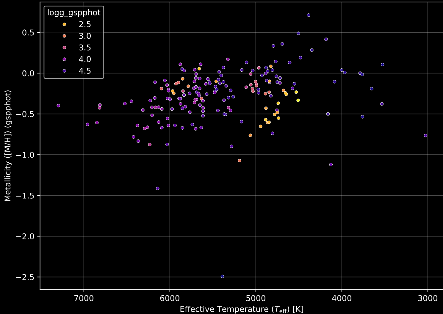
APOGEE DR17 Field: [029+77_MGA] Stellar Population Parameters (n= 184)
