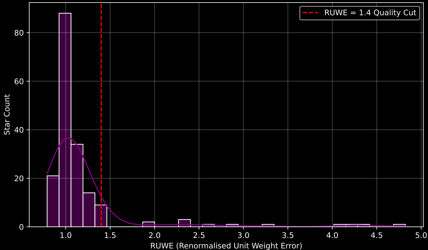
GAPOGEE DR17 Field [029+77_MGA] RUWE Distribution (n= 178)
